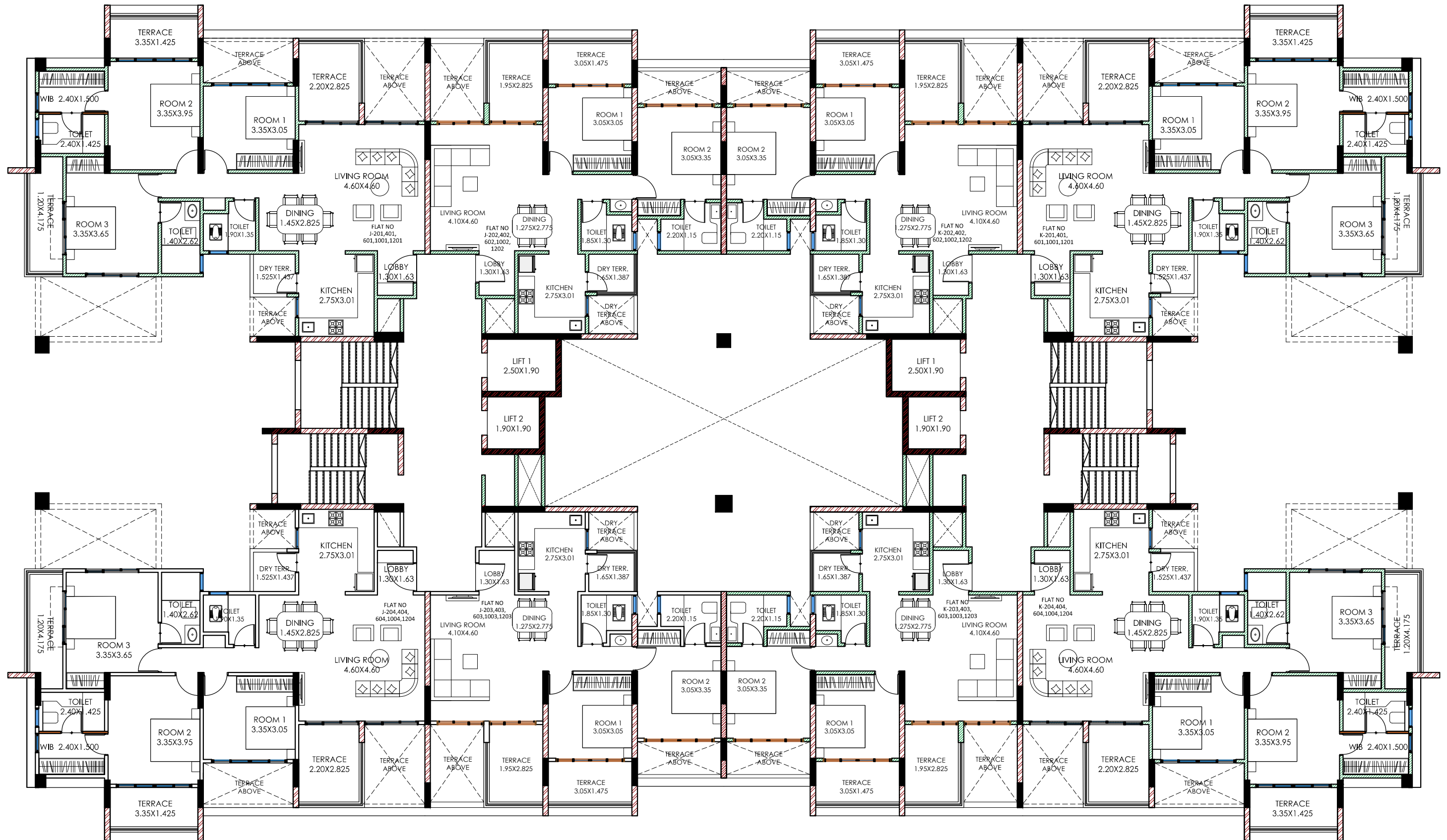
( J & K WING ) TYPICAL 2ND, 4TH, 6TH, 10, 12TH FLOOR PLAN
