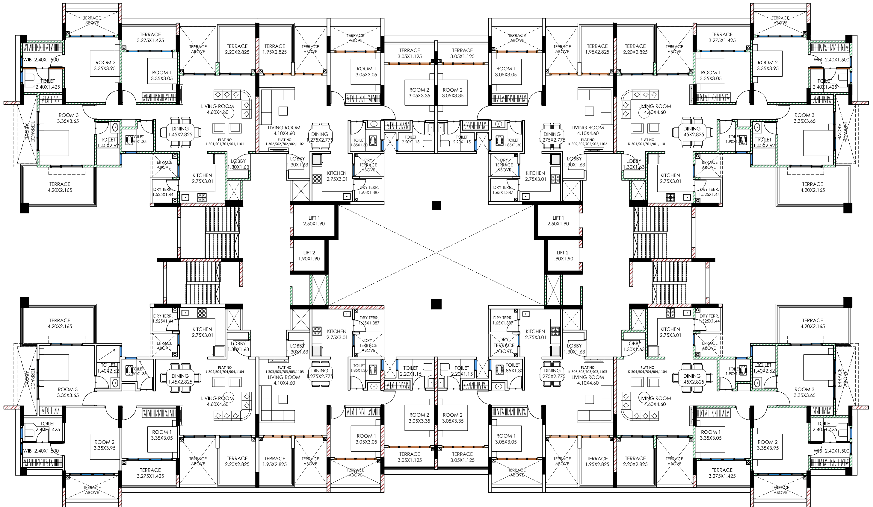
( J & K WING ) TYPICAL 3RD, 5TH, 7TH, 9TH, 11TH FLOOR PLAN
