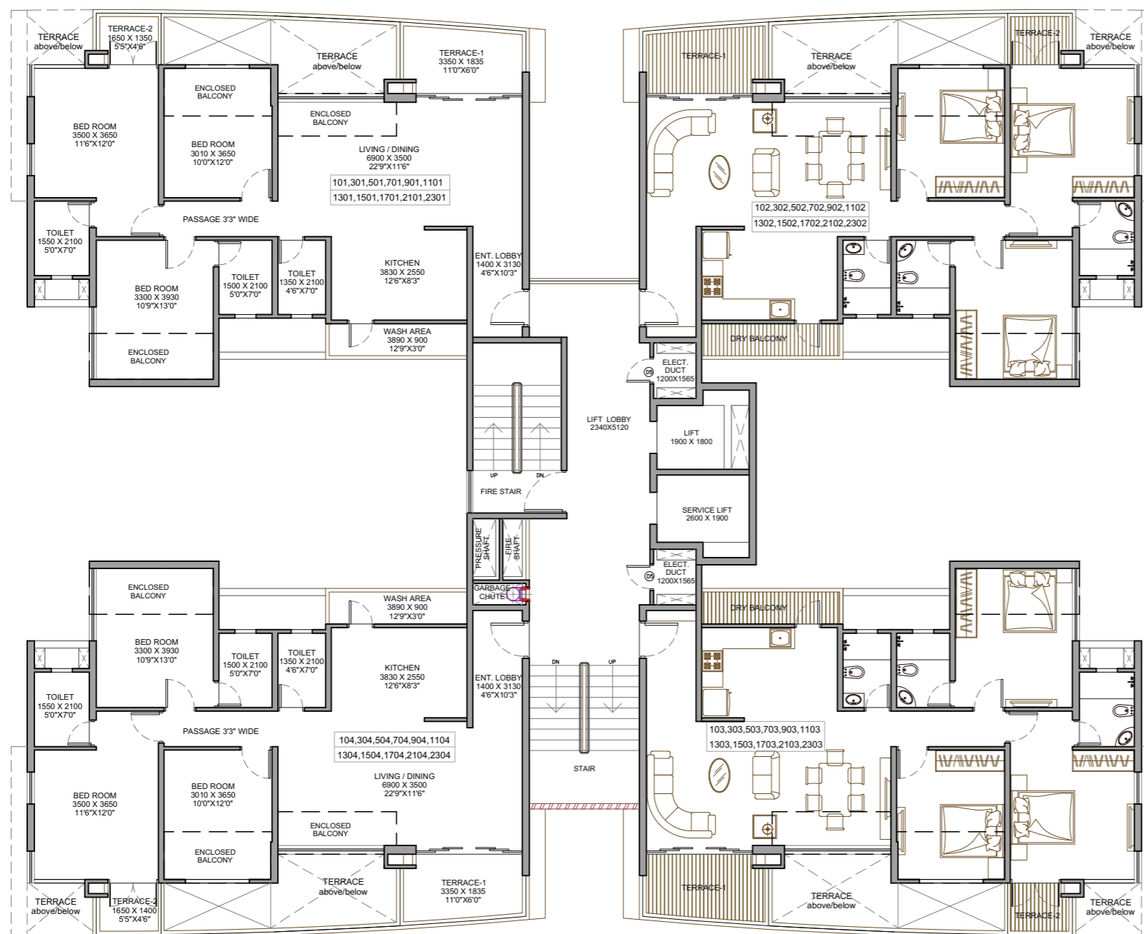
TYPICAL ODD FLOOR PLAN
